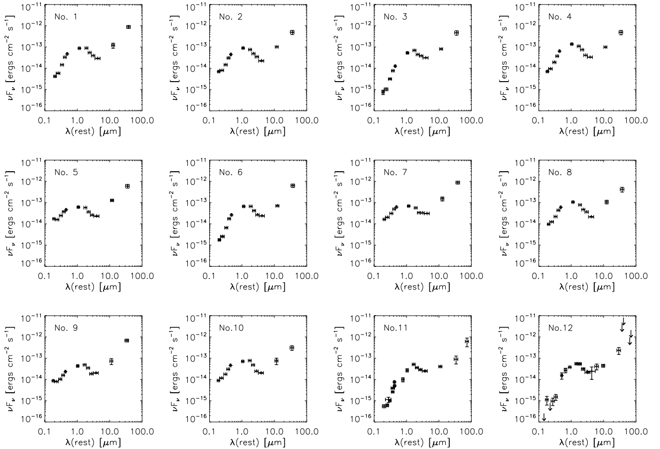
Figure 2. 0.1–100 \mu\text{m} SEDs of the 12 galaxies, illustrating \nu f_{\nu} ( \text{erg cm}^{-2} \text{s}^{-1} ) as a function of rest wavelength ( \mu\text{m} ).
