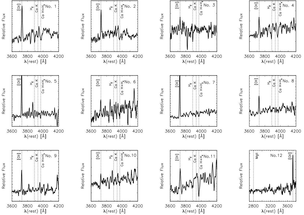
Figure 3. Optical spectra of the 12 galaxies. The relative flux densities (per Å) are plotted as a function of rest-frame wavelength (Å). The vertical lines mark the positions of Mg II at 2798 Å; [O II] at 3727 Å; Ca II H and K at 3968 and 3934 Å, respectively; Hζ at 3889 Å; and Hε at 3970 Å.
