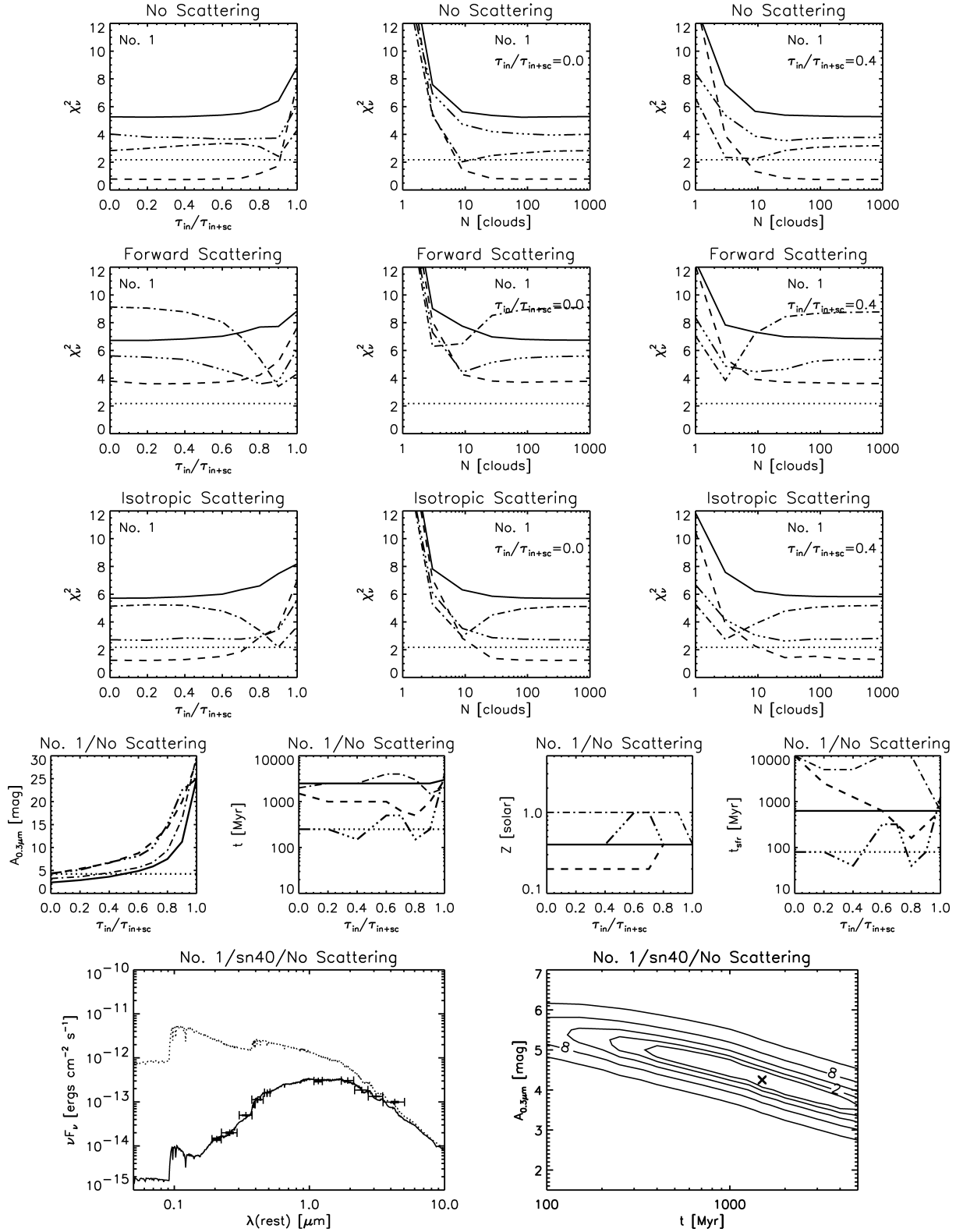
Figure 4. Results of the minimum \chi^2 analysis. The source number and the scattering property are indicated in each panel. The left-hand panels in the first three rows show \chi^2 for a uniform screen as a function of \tau_{in}/(\tau_{in} + \tau_{sc}) . The middle and right-hand panels in the first three rows represent a screen of N clumps for \tau_{in}/(\tau_{in} + \tau_{sc}) = 0 and \tau_{in}/(\tau_{in} + \tau_{sc}) = 0.4 , respectively. In case of no scattering, the scattering properties are no scattering for screen dust and forward scattering for internal dust. Solid lines represent 8–30 M_\odot SN dust, dashed 8–40 M_\odot SN dust, dash-dot MW dust, and dash-triple dot pseudo-MW dust, dotted the Calzetti dust. The fourth row panels show \tau_{in} + \tau_{sc} at 0.3 \mu m in magnitude A_{0.3\mu m} , the metallicity Z , the age t (yr), and the time-scale t_{SFR} as a function of \tau_{in}/(\tau_{in} + \tau_{sc}) . The bottom-row panels show the best-fitting SED along with the unreddened SED and the contour map of \chi^2 – \chi^2 (min). The full version of this figure is available with the online version of the paper – see Supporting Information.
