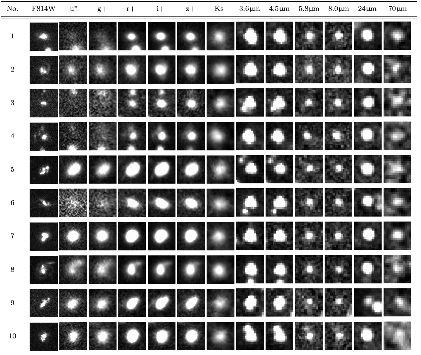
Figure 1. Postage stamp images of the 10 COSMOS galaxies. The size of each image is 4 \times 4 \text{ arcsec}^2 for F814W to Ks, 10 \times 10 \text{ arcsec}^2 for 3.6–8.0 \mu\text{m} , 20 \times 20 \text{ arcsec}^2 for 24 \mu\text{m} , and 50 \times 50 \text{ arcsec}^2 for 70 \mu\text{m} . North is up and east is to the left. Refer to Kawara et al. (2010) and Stern et al. (2006) for the images of No. 11 (SST J1604+4304) and No. 12 (HR10), respectively.
