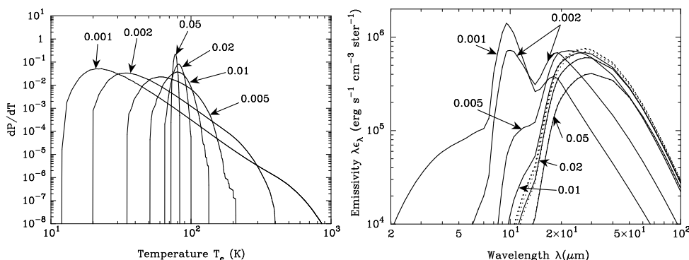
Figure 9. Temperature distribution functions of small astronomical silicate in the hot plasma with n_e = 10\text{cm}^{-3} and T_e = 10^7 K (left) and the emissivities (right) for given radii, where the radius is in units of \mu\text{m} .
