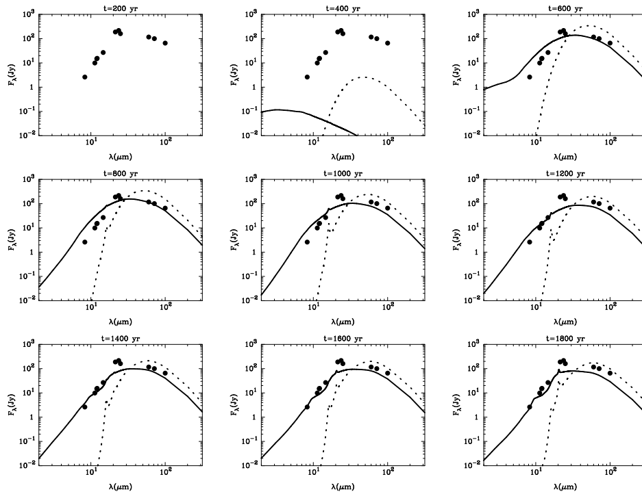
Figure 10. The time evolution of SEDs of Type IIb SNR for n_{\text{H}} = 1.0 \text{ cm}^{-3} with (solid curve) and without (dotted curves) stochastic heating. Closed circles are the flux densities subtracting the synchrotron radiation from the observed ones of Cas A (Hines et al. 2004)
