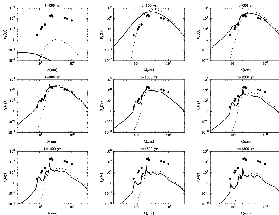
Figure 11. The same as Figure 10, but for n_{\text{H}} = 10.0 \text{ cm}^{-3}
