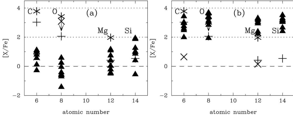
Figure 2. Abundances of C, O, Mg and Si relative to Fe in the dense shell of SN II remnants for n_{\text{H},0} = 0.1 and 1 \text{ cm}^{-3} (filled triangles); (a) derived from the elemental composition of the grains piled up in the shell, and (b) derived from the elemental composition of the piled-up grains and the gas outside the innermost Fe layer. For observational data of HMP and UMP stars, the 3-D corrected abundances are adopted and are denoted by plus (HE0107-5240 with [\text{Fe}/\text{H}] = -5.62 , Collet et al. 2006), asterisk (HE1327-2326 with [\text{Fe}/\text{H}] = -5.96 , Frebel et al. 2008), and cross (HE0557-4840 with [\text{Fe}/\text{H}] = -4.75 , Norris et al. 2007).
