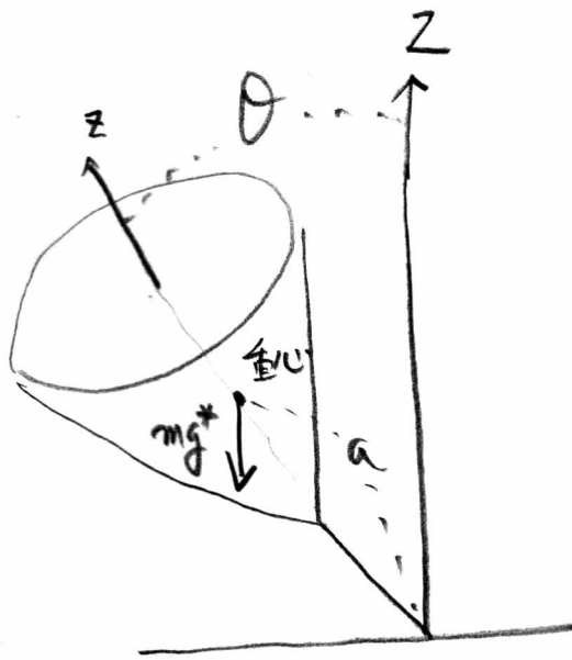
Figure 4: 対称独楽
