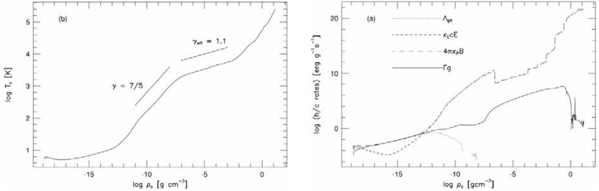
Figure 4.12: (Left) Relation between density and temperature at the center of the cloud. (Right) Cooling and heating rates, which are calculated for the cloud center are plotted against the density.
