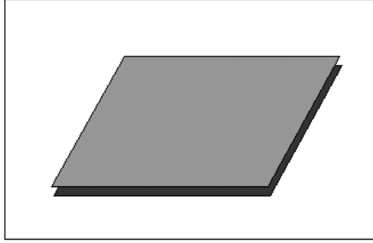
Figure 2.3: Thin disk.
