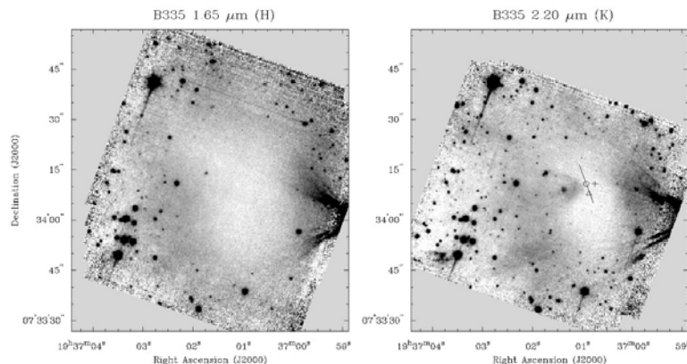
Figure 1.8: Near infrared images of B335, which is a Class 0 source.
