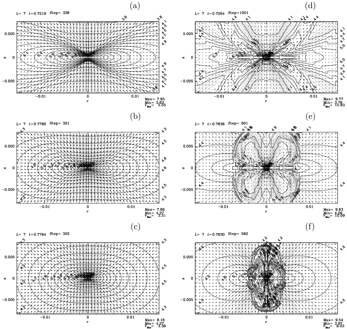
Figure 4.17: Difference in models with the same rotation speed \Omega = 2 \times 10^{-14} \text{ rad s}^{-1} but different magnetic field strength ((a) and (d): B_c = 10\mu\text{G} , (b) and (e): 3\mu\text{G} , and (c) and (f): 1\mu\text{G} ).
