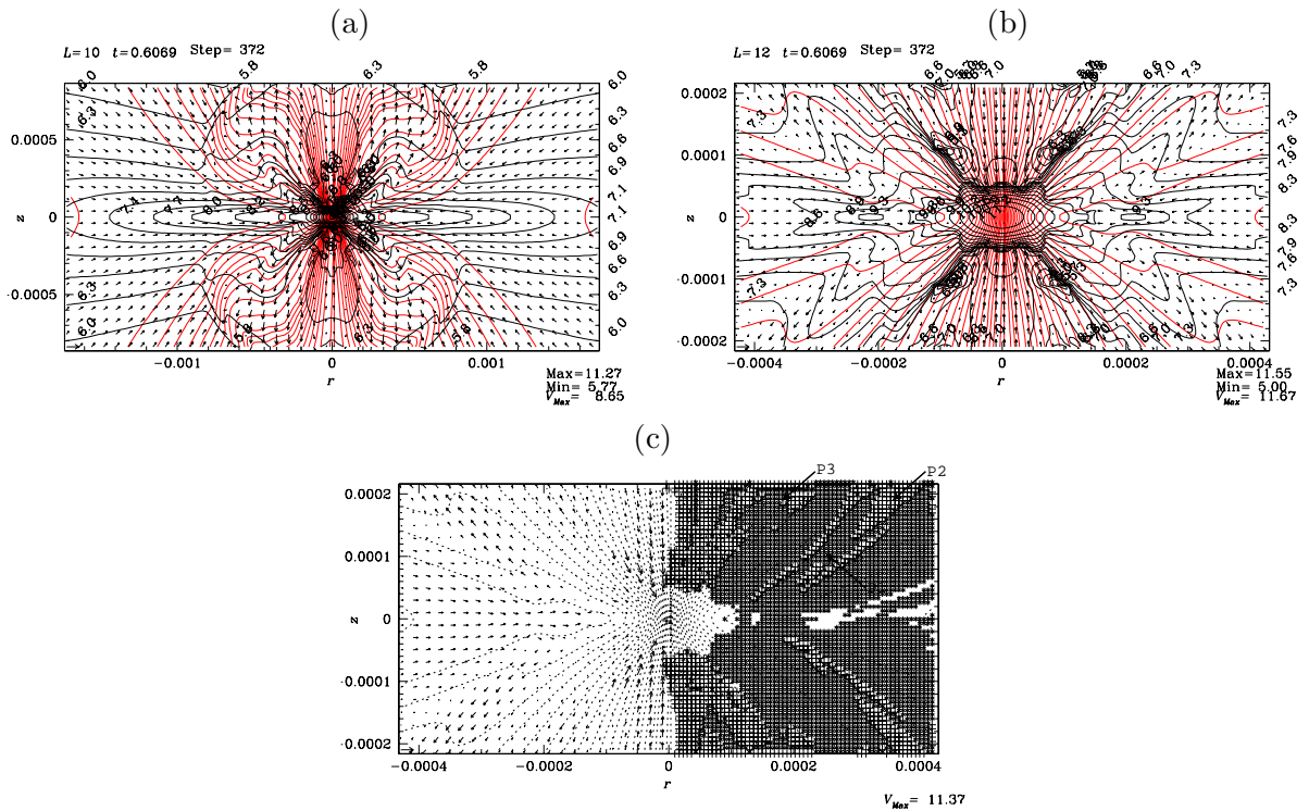
Figure 4.16: Continuation of the evolution shown in Fig.4.15. Snapshots at the time of 0.6069 \tau_{\text{ff}} = 1.066 \text{ Myr} just \sim 500 \text{ yr} after from Fig.4.15. Panel (a) plots the structure of L10 which is similar to Fig.4.15 (c). Spherical region inside \sim 1.2 \times 10^{-3} H has been swept by the outflow. Panel (b) is a snapshot of L12 grid which has 4-times finer spatial resolution than L10 (a). In panel (c), we plotted magnetic force dominated region with '+', centrifugal force dominated with '*', and thermal pressure force dominated with blank ' '.
