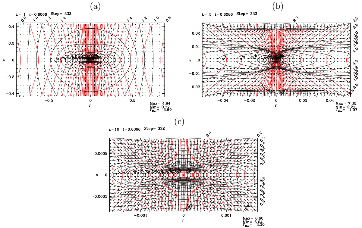
Figure 4.15: \Omega_c = 10^{-13}\text{rad s}^{-1} , B_c = 10\mu\text{G} , \rho_c = 10^4\text{H}_2\text{ cm}^{-3} , and c_s = 190\text{m s}^{-1}(T/10\text{K}) . Snapshots at the time of 0.6066\tau_{\text{ff}} = 1.061\text{Myr} represented in different levels are shown: L1 (upper-left), L5 (upper-right), and L10 (bottom). The actual size of the frames of L5 (upper-right) and L10 (bottom) are, respectively, 1/16 and 1/512 smaller than that of L1 (upper-left). Magnetic field lines (dotted lines) and isodensity contours (solid lines) are presented as well as the velocity vectors by arrows.
