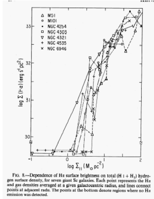
Figure 3.2: Distributions of \Sigma_{\text{SF}} and \Sigma_{\text{gas}} . (Left:) Relation between \Sigma_{\text{SF}} and \Sigma_{\text{gas}} for an Sc galaxy NGC 4254 and an Sb galaxy NGC 2841. (Right:) Relation between \Sigma_{\text{SF}} and \Sigma_{\text{gas}} for various galaxies. These are taken from Figs.7 and 8 of Kennicutt (1989).
