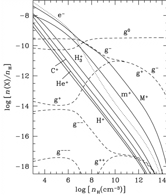
Figure 4.3: Ionization fractions X/n_{\text{H}} are plotted against the number density n_{\text{H}} . The ionization rate of an \text{H}_2 molecule by cosmic rays outside the cloud is taken \zeta_0 = 1 \times 10^{-17} \text{s}^{-1} . 20% of C and O and 2% of metallic elements are assumed to remain in the gas phase and the rest in grains.
