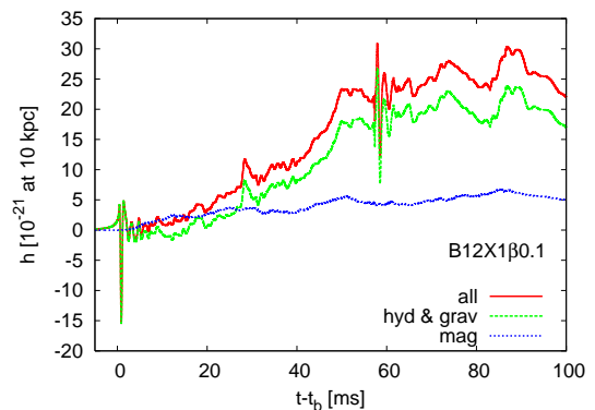
Figure 2: Amplitude of the gravitational wave as a function of time (Red line). Green and blue lines depict the contributions of hydrodynamical part and magnetic part, respectively.
