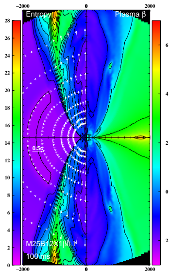
Figure 1: Time snapshot of MHD explosion: Entropy[kB] and plasma \beta are shown in the left and right panel, respectively.
